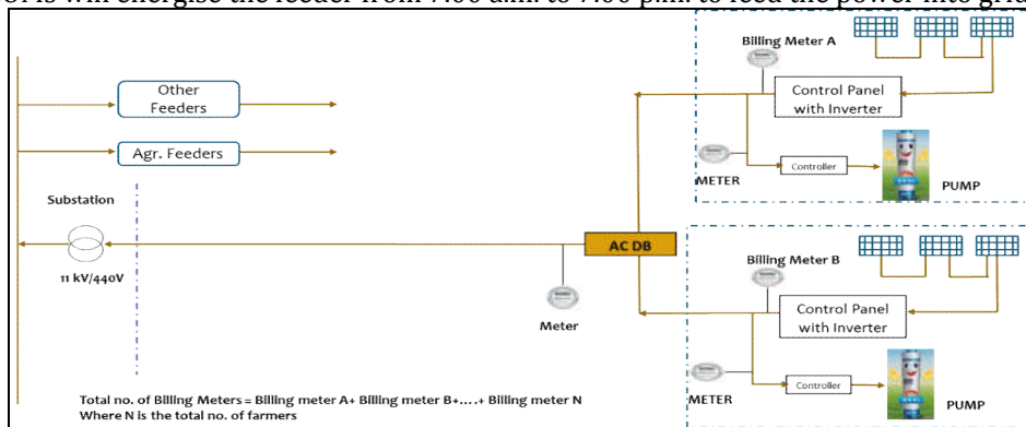
Figure 1: System Configuration of Proposed Solar PV based Mini Grid
