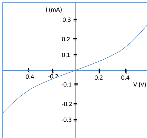
Fig. 5: I-V characteristics between Y-S and stainless steel.
