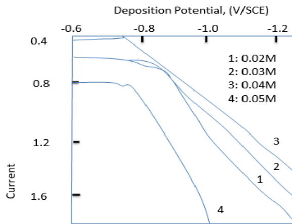
Fig. 2: The polarization curves for various sulphur ion concentrations on to a stainless-steel substrate.
