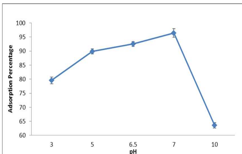
Figure 1. Effect of various pH on the adsorption percentage of lead (Adsorbent quantity =10 g/L, Contact time=30 min, Initial concentration of lead=10 mg/L)
