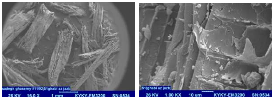
Figure 9. SEM images before adsorption of metal by myrtaceae sawdust with 16X and 1KX magnifications
