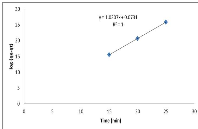
Figure 8. Second-degree adsorption kinetic model
