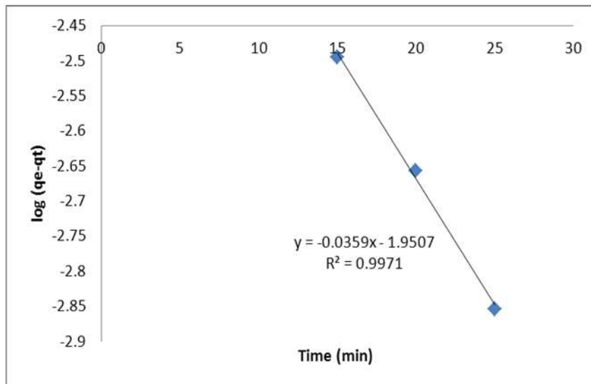
Figure 7. First-degree adsorption kinetic model
