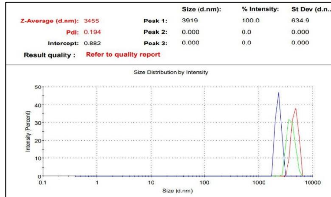
Fig. 1. Particle size distribution curve of BASM TSM microspheres
