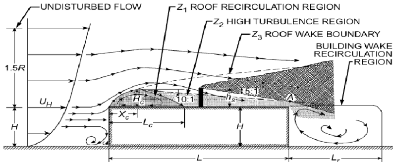
Figure 5. The flow pattern around the building with chimney Wilson (1979)
