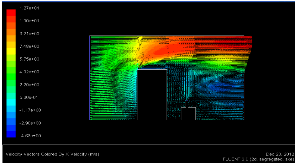
Figure 11. Velocity vectors in X direction
