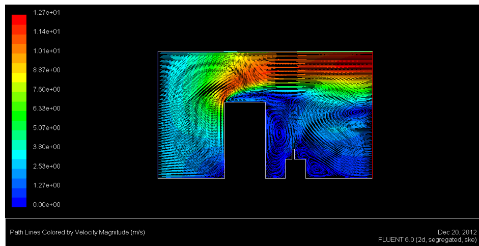
Figure 13. Flow patterns in Models
