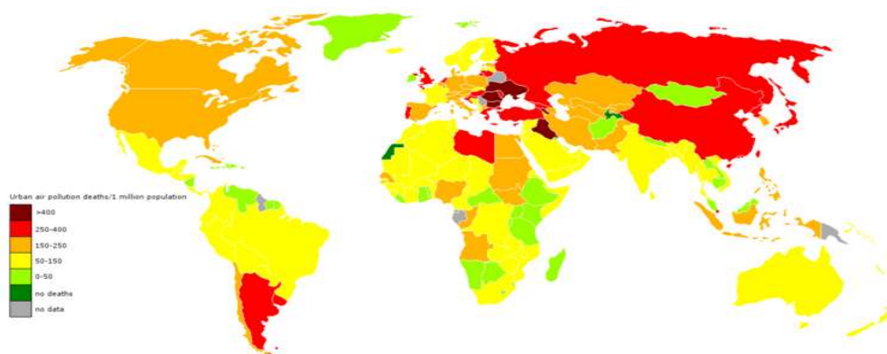
Figure 2. Distribution of deaths caused by pollution in 2004
