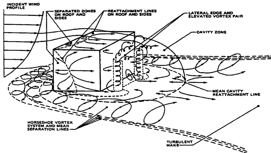
Figure 3. The flow pattern around the building with cutting edge Hosker (1979)
