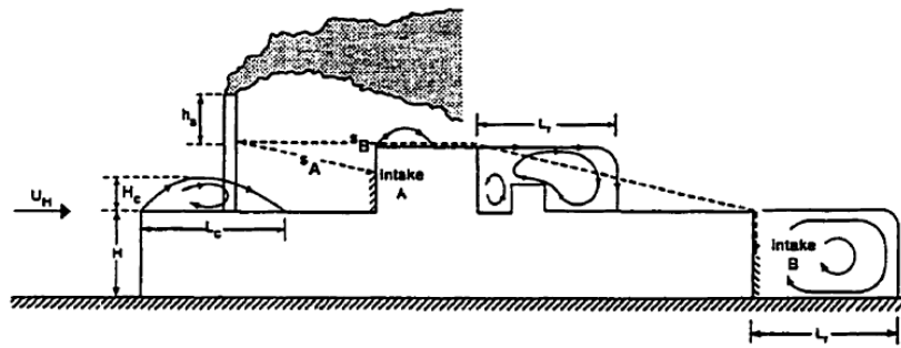
Figure 6. The flow pattern around the building of complex geometry (ASHRAE Handbook-1997 Fundamentals15.2) [13]
