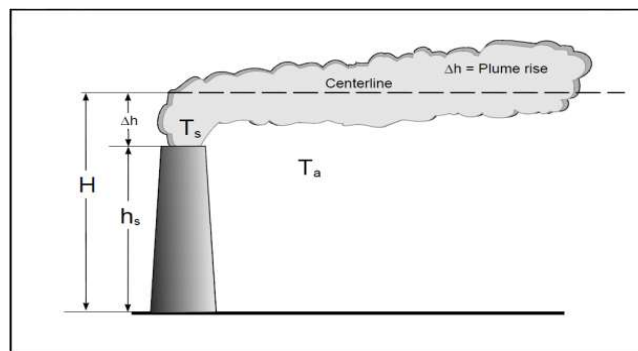
Figure 7. Effective chimney height
