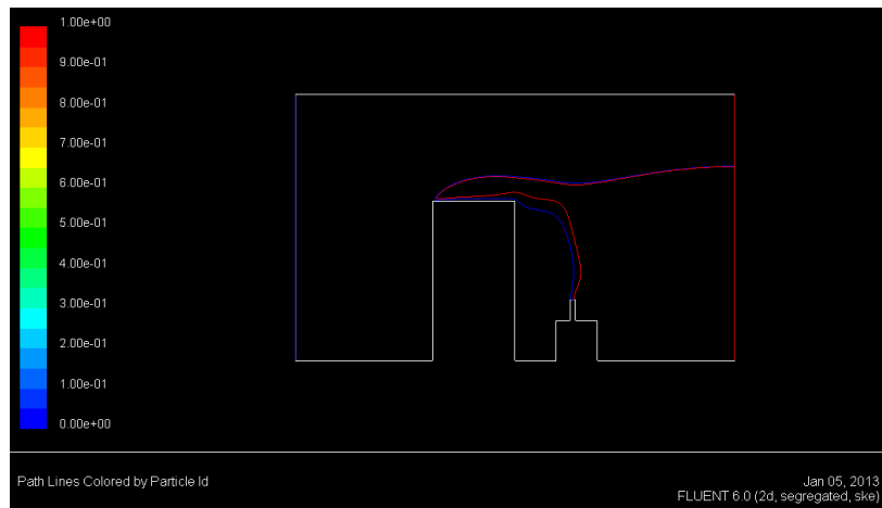
Figure 14. Flow pattern of smoke from the chimney
