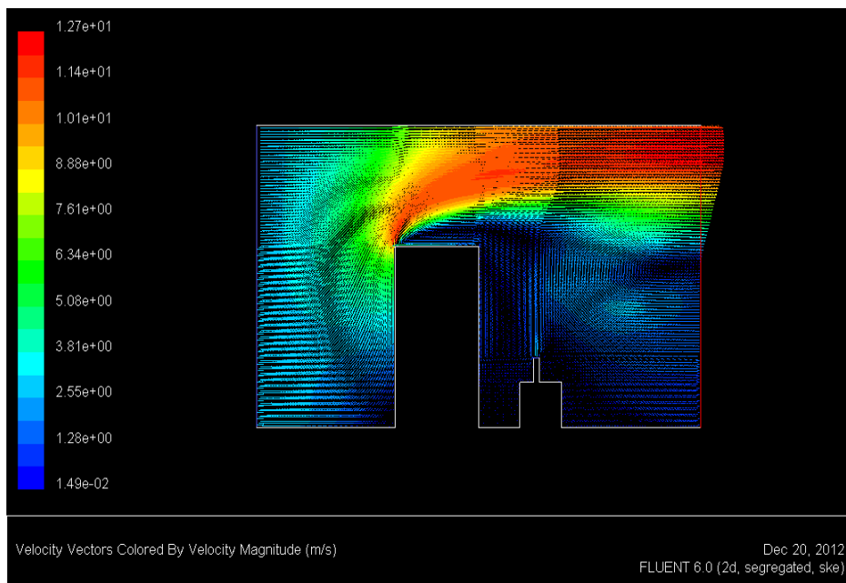
Figure 10. Velocity vectors in the model.
