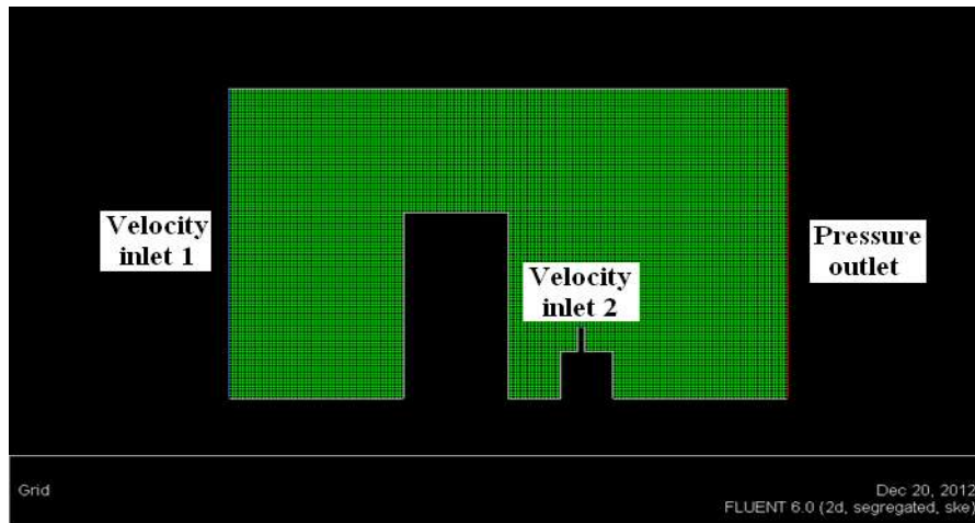
Figure 9. Model geometry, mesh and boundary conditions applied in the model.
