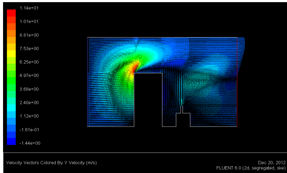
Figure 12. Velocity vectors in Y direction
