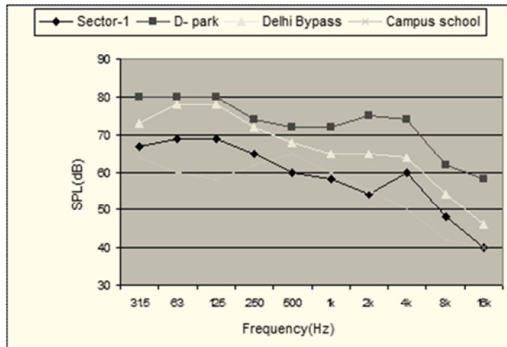
Figure (3): Power spectra in residential (Sector-1), commercial (D-park), traffic junction (Delhi bypass) and silent areas (Campus school)
