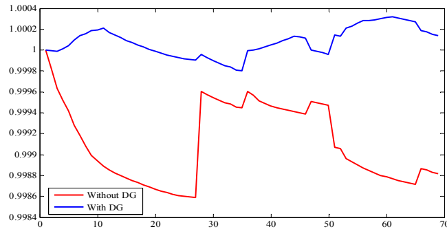
Fig 3: Voltage profile with and without DGs in 69 bus system using PSO
