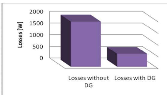
Fig 2: Bar Losses profile with & without DG in 69 bus system
