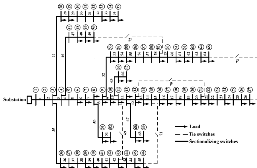
Fig 1: Single line diagram for a 69-bus radial distribution system
